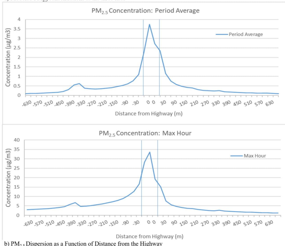
FIGURE 3 a) Modeled PM 2.5 Concentrations at the three sites b) PM 2.5 Dispersion as a Function of Distance from the Highway
