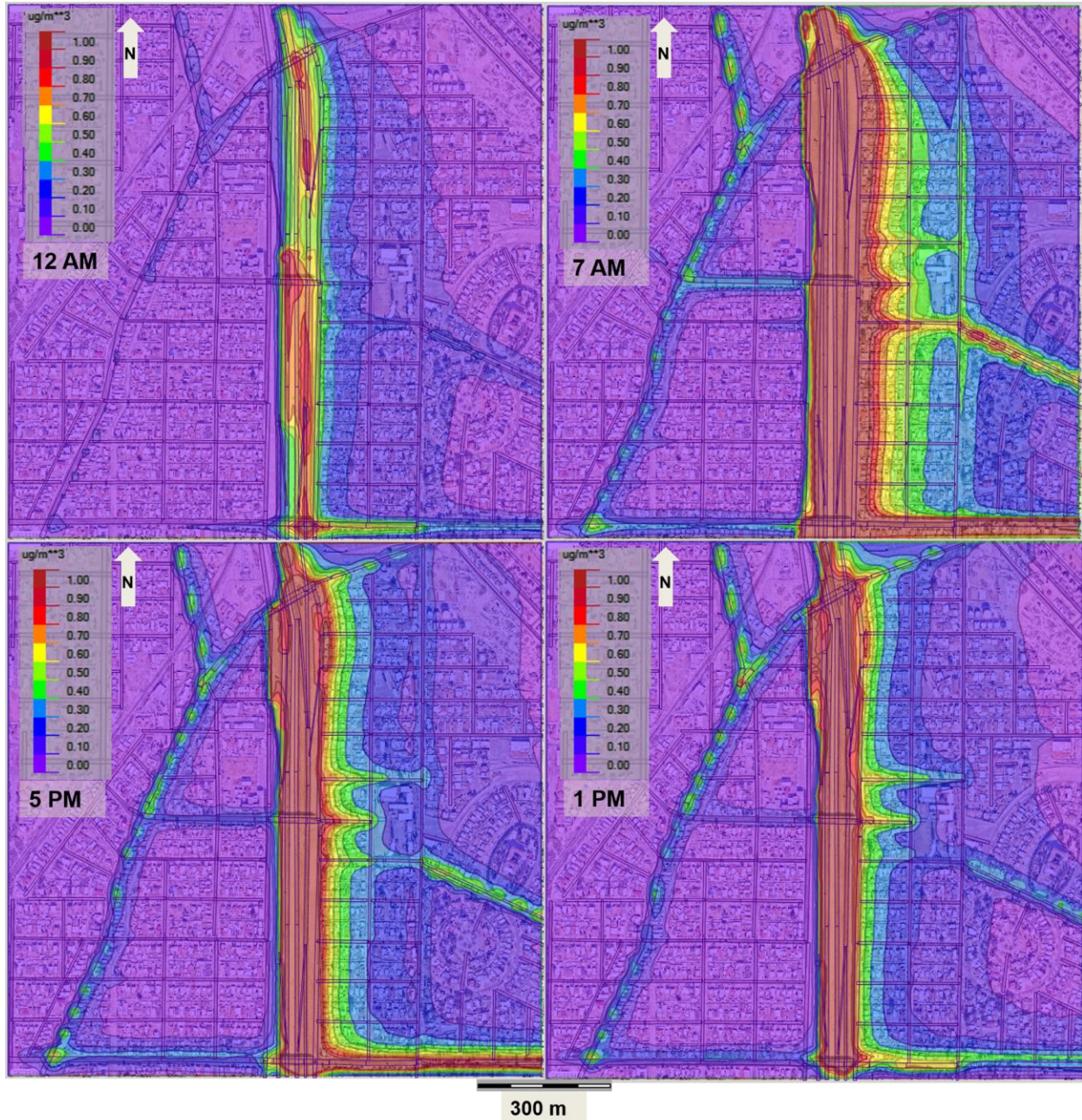
Figure 37 PM 2.5 Hourly Concentrations at Different Peak Hours, Friday May 18 th
