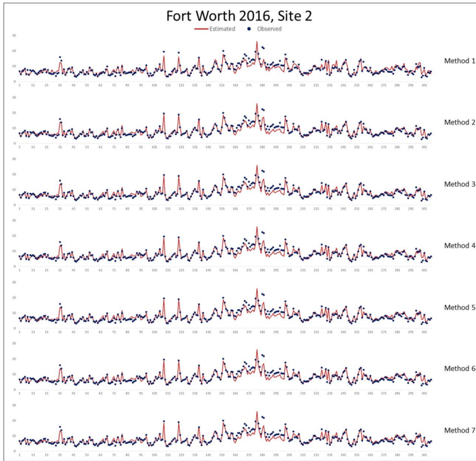
455 FIGURE 3 Comparison of predicted vs observed PM 2.5 concentrations by different 456 methods
