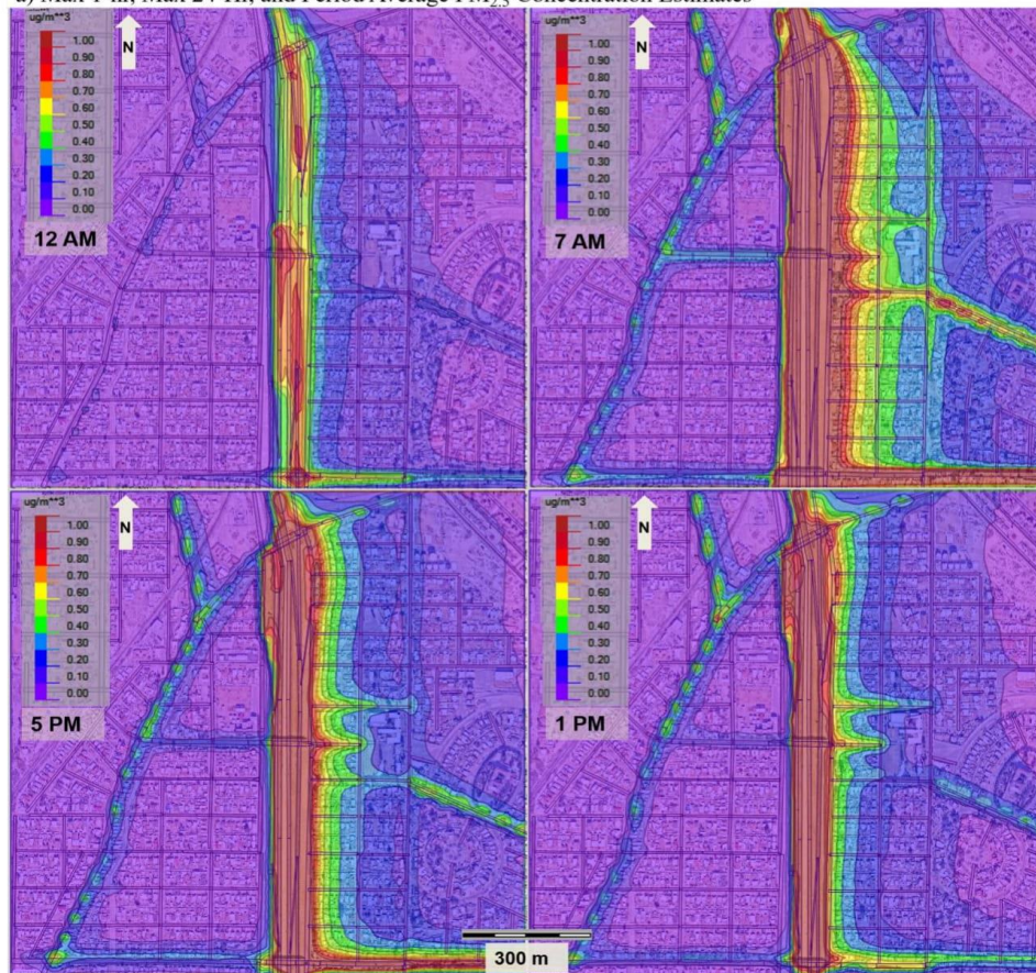
b) Max 1-hr, Max 24-Hr, and Period Average PM 2.5 Concentration Estimates
