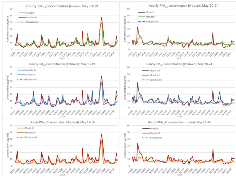
1 2 FIGURE 5 Comparison of Model Results and On-Site Monitoring: Hourly PM 2.5 3 Concentrations
