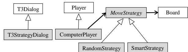
Fig. 3. Extending with strategies, new classes shown in gray
