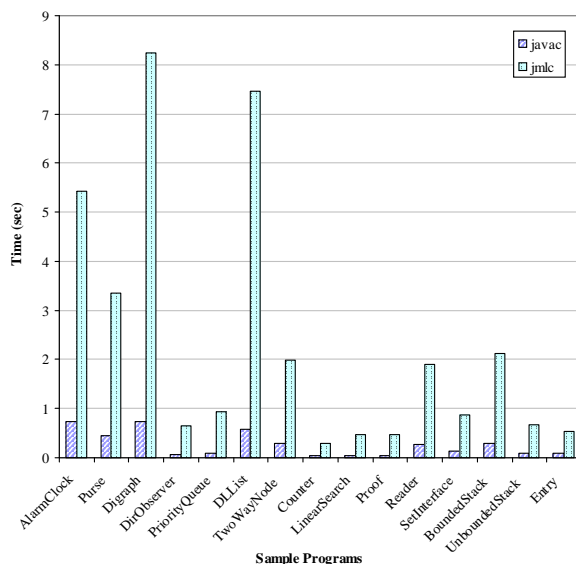
Figure 2. Compilation times of jmlc and javac
